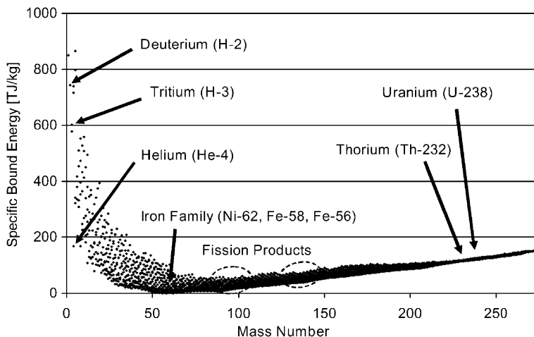
Fig. 1. Nucleus-bound energy of known nuclides (Ni-62 = 0).
