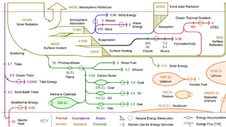
Fig. 2. Global reservoirs, flux, and anthropogenic destruction of exergy.
