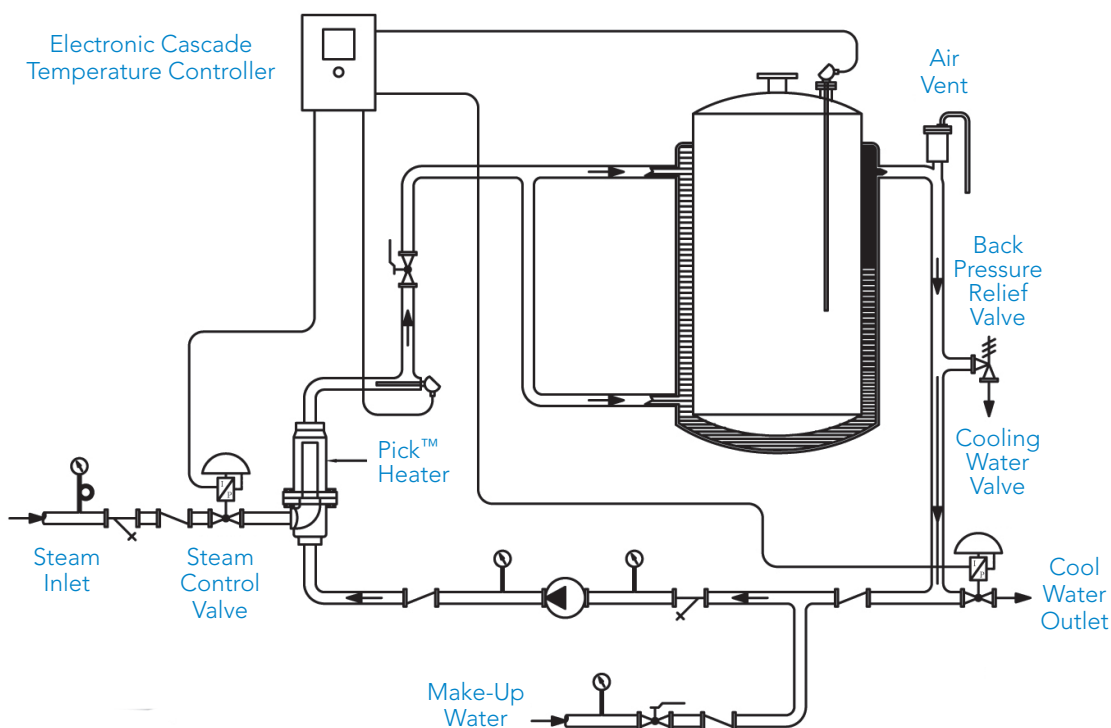
Figure 5. Typical jacketed heating system with Pick™ DSI heater
