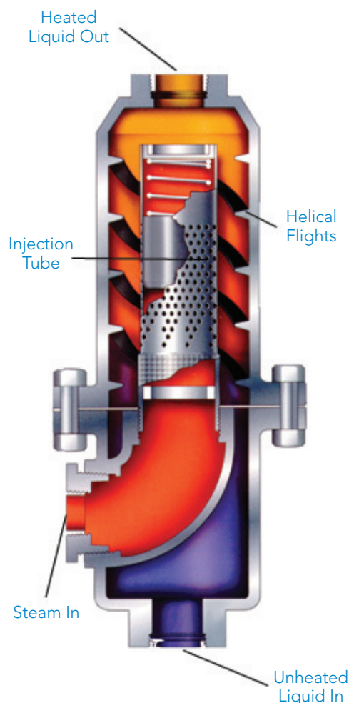
Figure 3. Multiple Orifice DSI Heater
