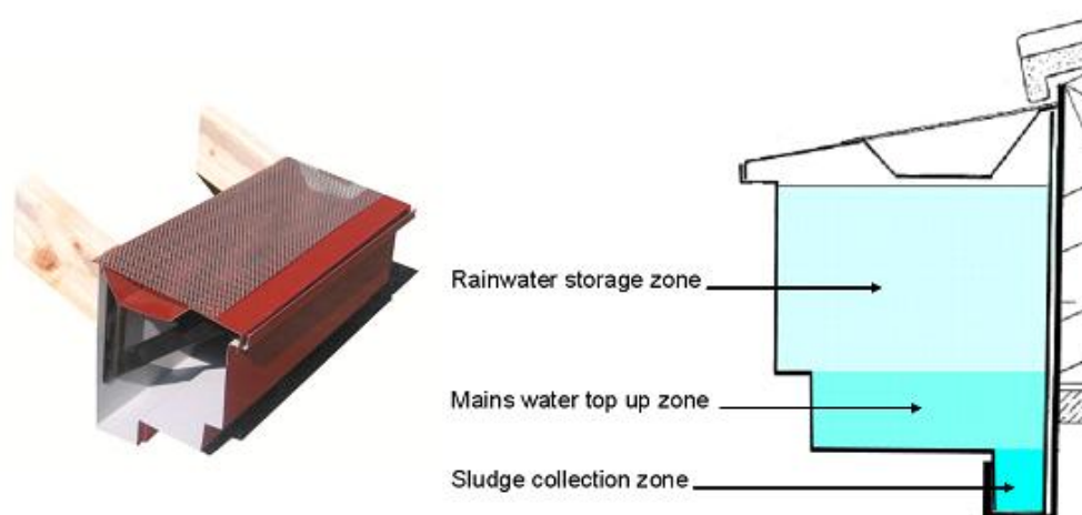
Figure 1. Cutaway section of medium sized storage gutter plus diagram showing storage zones.
