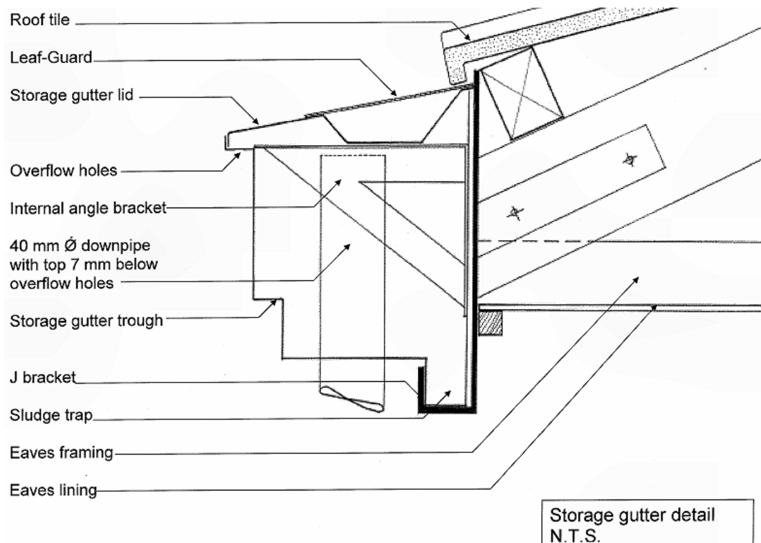
Figure 2. Gutter section showing downpipe and fixing brackets.
